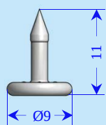
單針鋁鉚釘 Single-pin aluminum rivet
